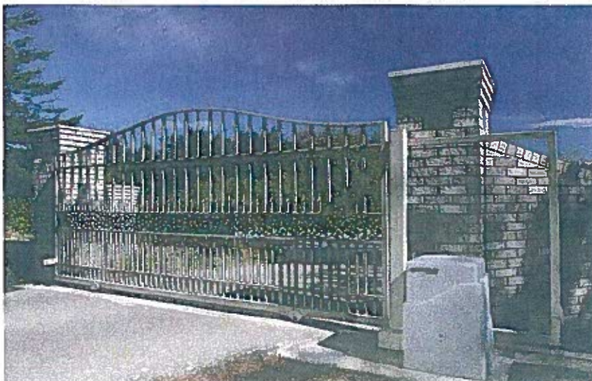
SlideWinder 38 1 hp 200 lb. pull force 2,000 lb. max gate weight 38' max gate travel UL Class I - IV 115/208-230 single phase 50 or 60 Hz
