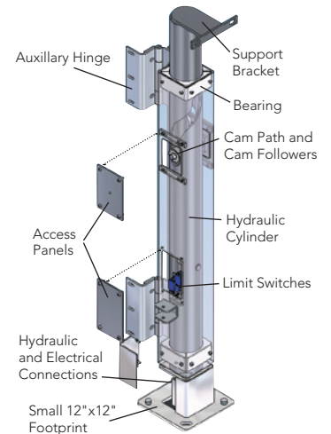
SwingRiser™ Post
