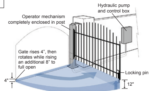
SwingRiser™ Post
